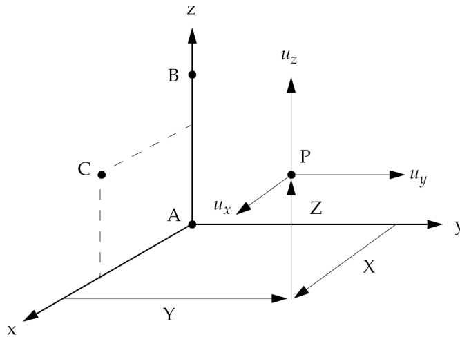
Figure 13-6. CORD2R Definition
