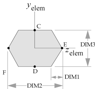
TYPE="HEXA"
