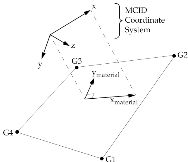
Figure 13-12. MCID Coordinate System Definition
