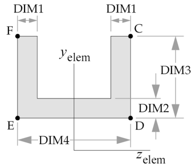
TYPE="CHAN2"
