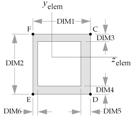
TYPE="BOX1"
