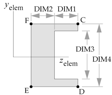
TYPE="CHAN1"
