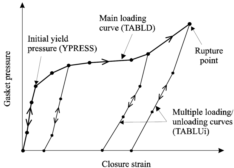
Figure 16-2. Pressure-Closure Relationship for a Gasket Material
