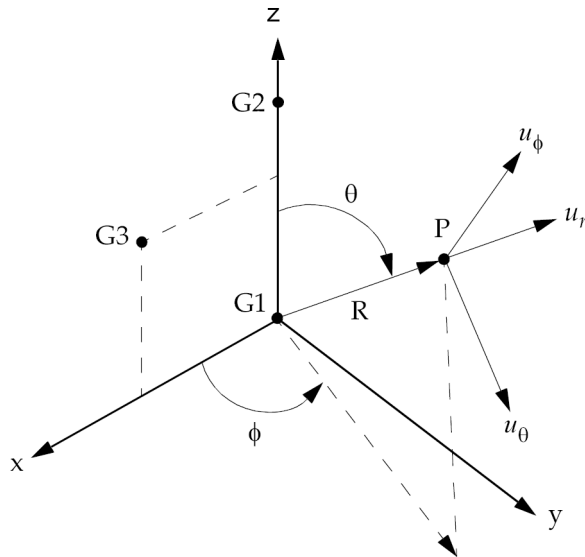
Figure 13-4. CORD1S Definition
