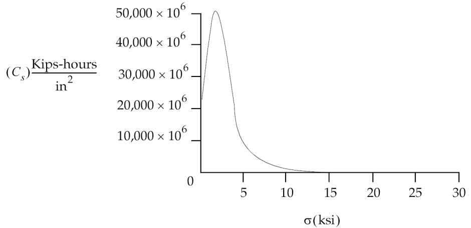
Figure 13-28. C s Versus s Example for CREEP
