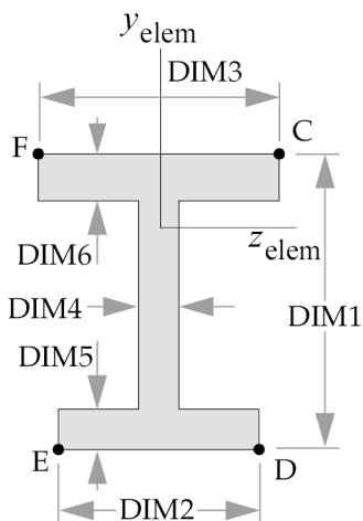
TYPE="I"
