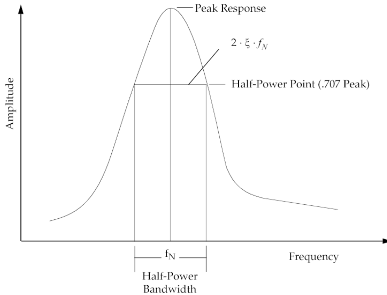
Figure 15-5. Half-Power Bandwidth Definition
