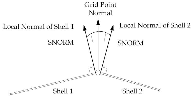
Figure 7-1. Unique Grid Point Normal for Adjacent Shell Elements
