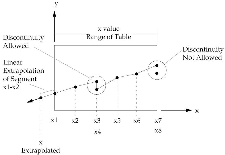
Figure 19-5. Example of Table Extrapolation and Discontinuity
