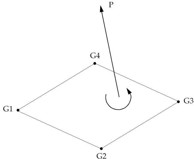
Figure 17-16. Pressure Convention for Quadrilateral Surface of Surface Elements and/or the Faces of Solid Elements
