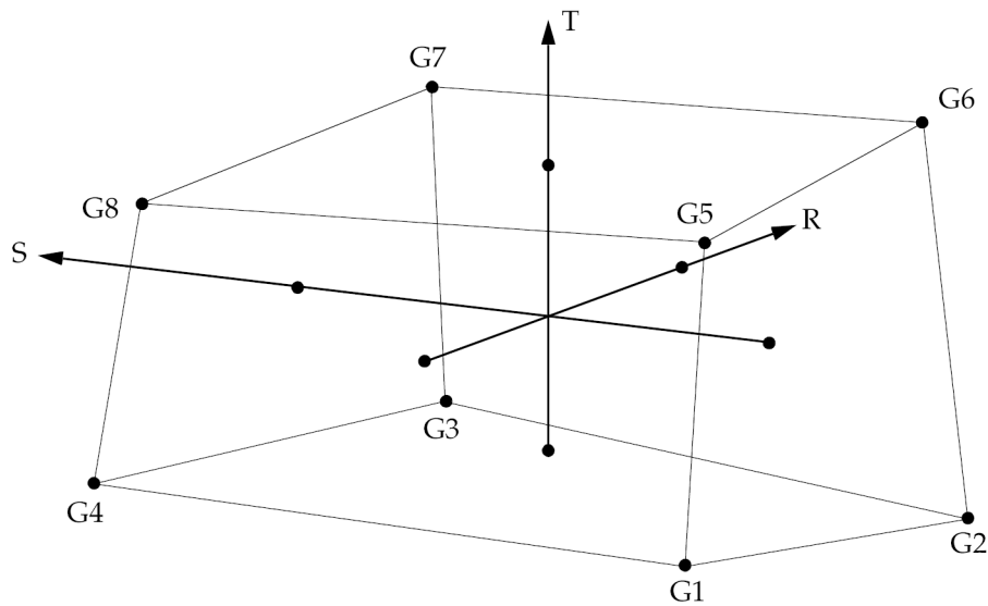
Figure 12-30. CHEXA Element R, S, and T Vectors
