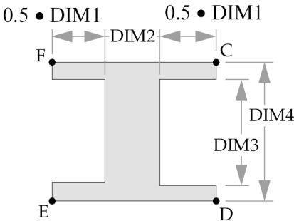
TYPE="I1"
