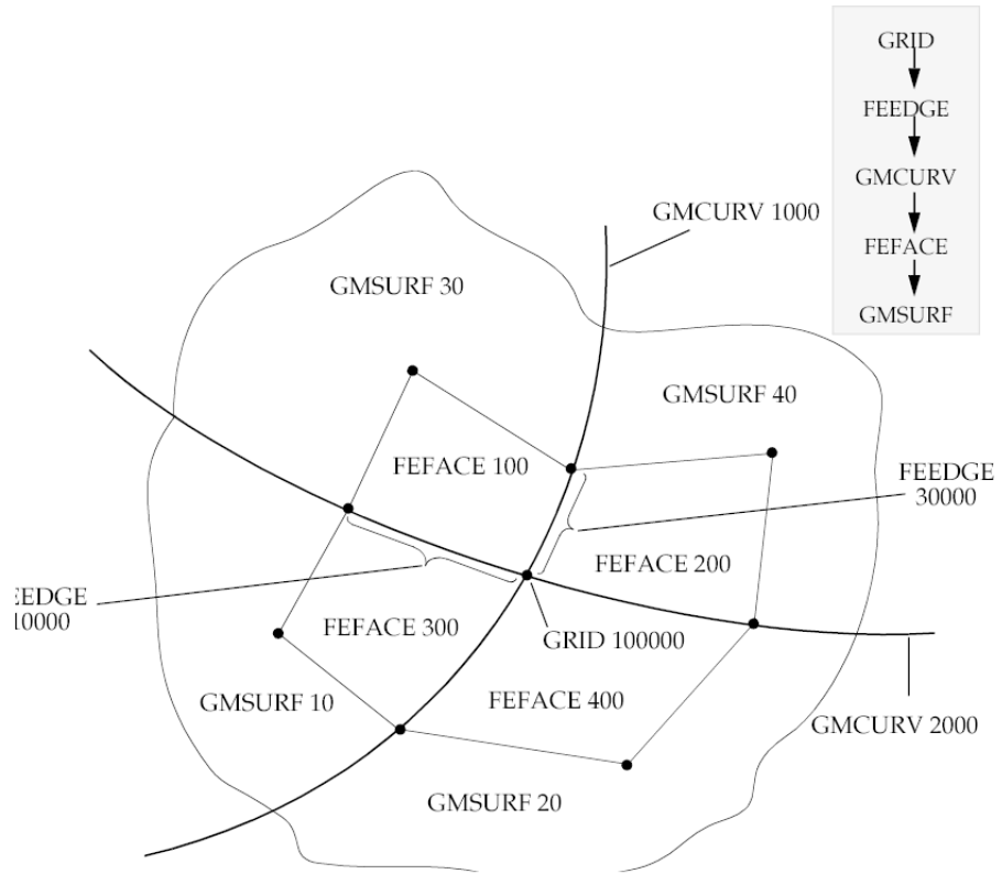
Figure 15-6. Use of Multiple Surface and Curves
