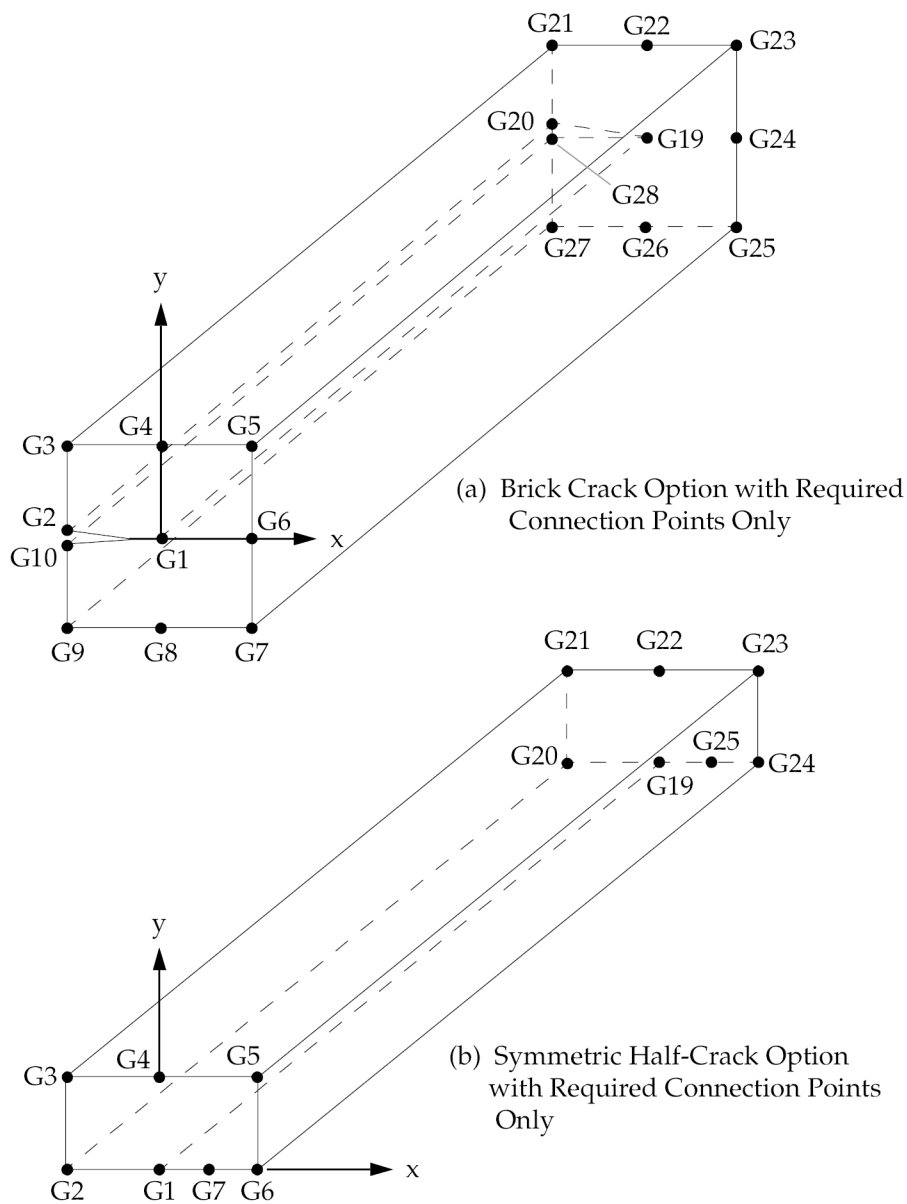
Figure 13-23. CRAC3D Solid Crack Tip Element with Required Connection Points Only
