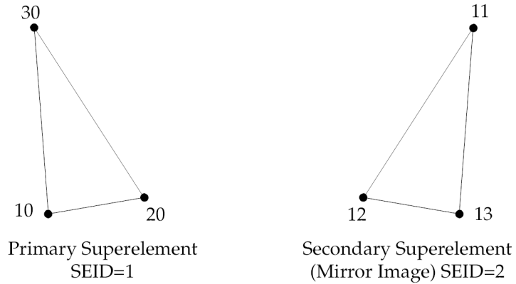
Figure 18-4. Grid Point Correspondence Between Primary and Secondary Superelements
