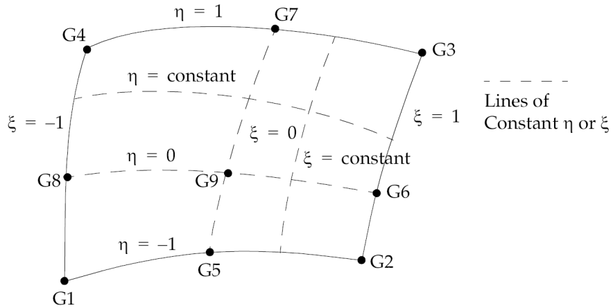
Figure 13-11. CQUAD Element Coordinate System
