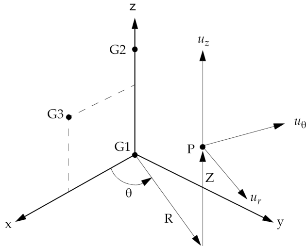
Figure 13-2. CORD1C Definition
