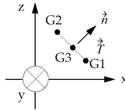
Figure 12-23. Normal Vector for CHBDYG Element of Type “REV”
