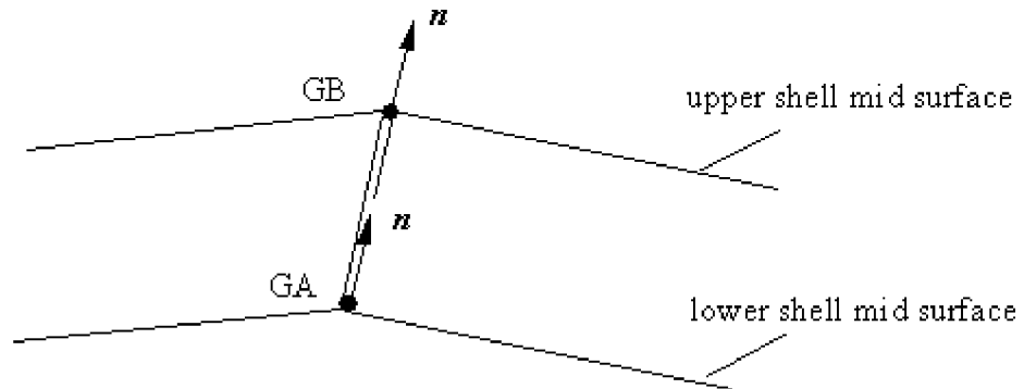
Figure 13-53. Point-to-Point Connection Defined with Format ALIGN
