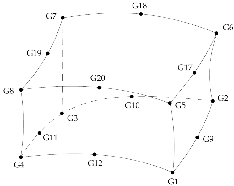
Figure 12-22. CHACBR Element Connection
