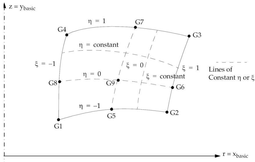
Figure 13-17. CQUADX Element Coordinate System
