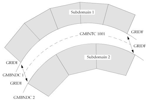
Figure 15-9. Geometric Interface Element Definition (Exploded View)
