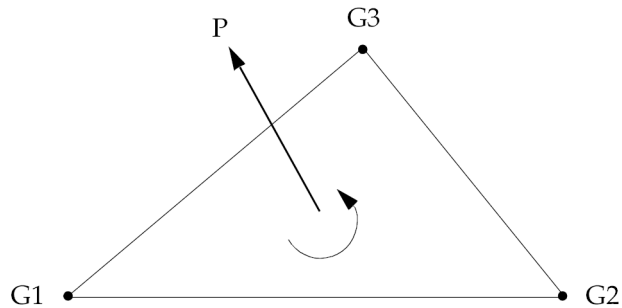
Figure 17-15. Pressure Convention for Triangular Surface of Surface Elements and/or the Faces of Solid Elements
