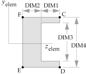
TYPE="CHAN1"
