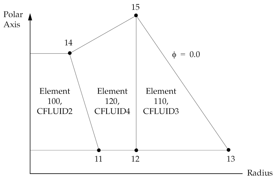
Figure 12-19. CFLUIDi Examples
