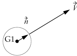
Figure 12-26. Normal Vector for CHBDYP Element of Type "POINT" (See Remarks 4 and 5.)
