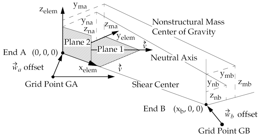
Figure 12-11. CBEAM Element Geometry System (Non p-adaptive)
