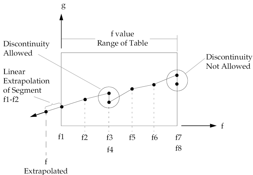
Figure 19-9. Example of Table Extrapolation and Discontinuity
