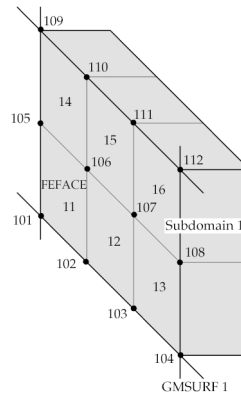
Figure 15-8. Surface Boundary Definition
