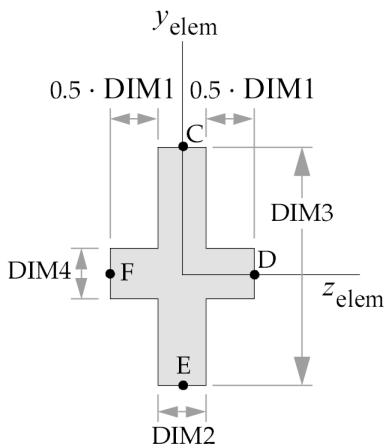
TYPE="CROSS"
