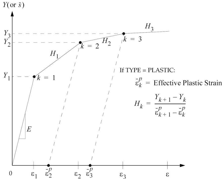
Figure 16-4. Stress-Strain Curve Definition When TID Is Specified in Field 3
