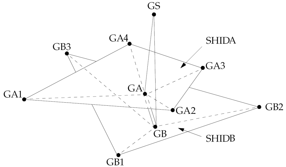
Figure 13-51. Patch-to-Patch Connection Defined with Format GRIDID or ELEMID
