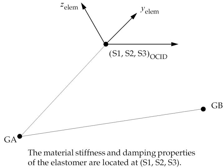
Figure 12-17. Definition of Offset S1, S2, S3
