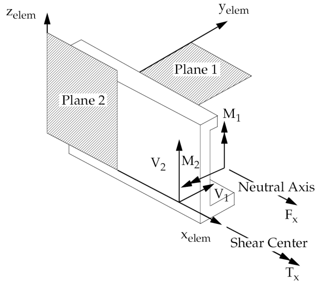
Figure 12-13. CBEAM Internal Element Forces and Moments
