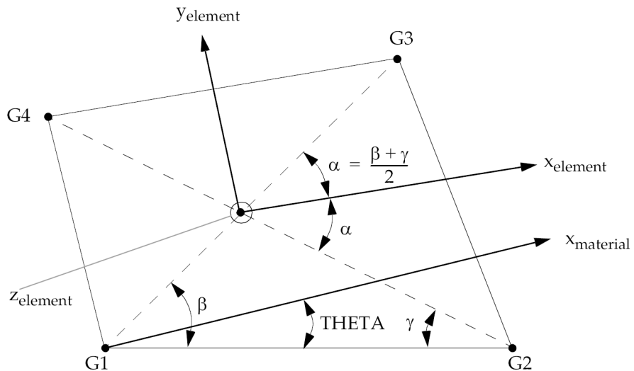
Figure 13-16. CQUADR Element Geometry and Coordinate Systems
