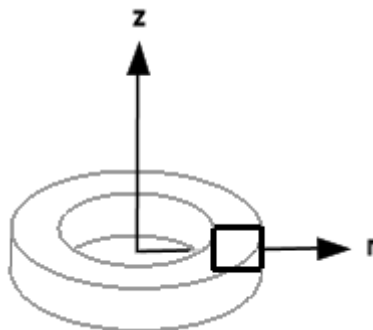
Figure 13-18. CQUADX4 Element Idealization
