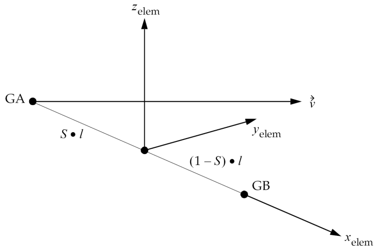
Figure 12-16. CBUSH Element
