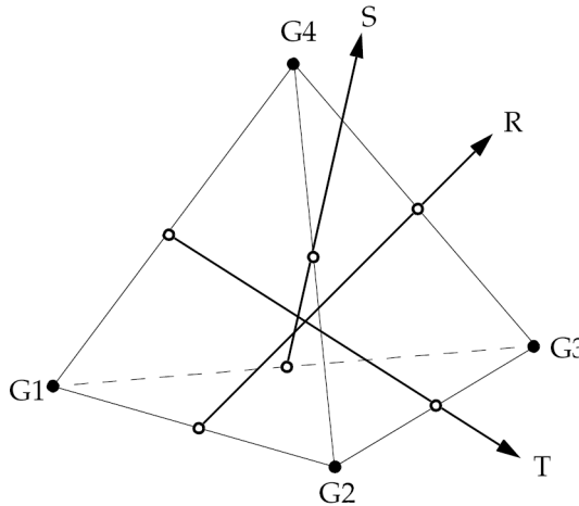
Figure 13-33. CTETRA Element R, S, and T Vectors
