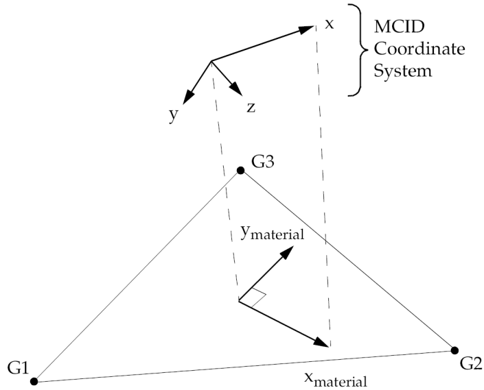
Figure 13-40. MCID Coordinate System Definition
