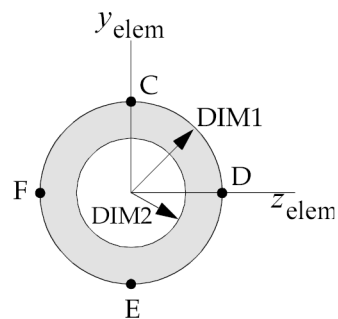
TYPE="TUBE"
