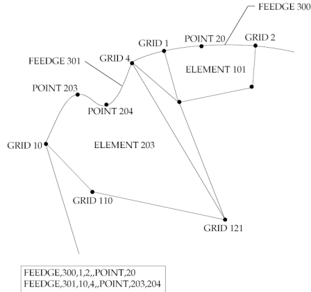
Figure 15-2. Specifying Geometry Using GEOMIN=POINT Method
