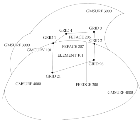
Figure 15-3. Face Edge Common to Two Surfaces
