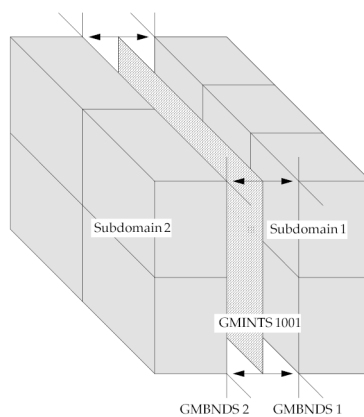
Figure 15-10. Geometric Interface Element Definition (Exploded View)
