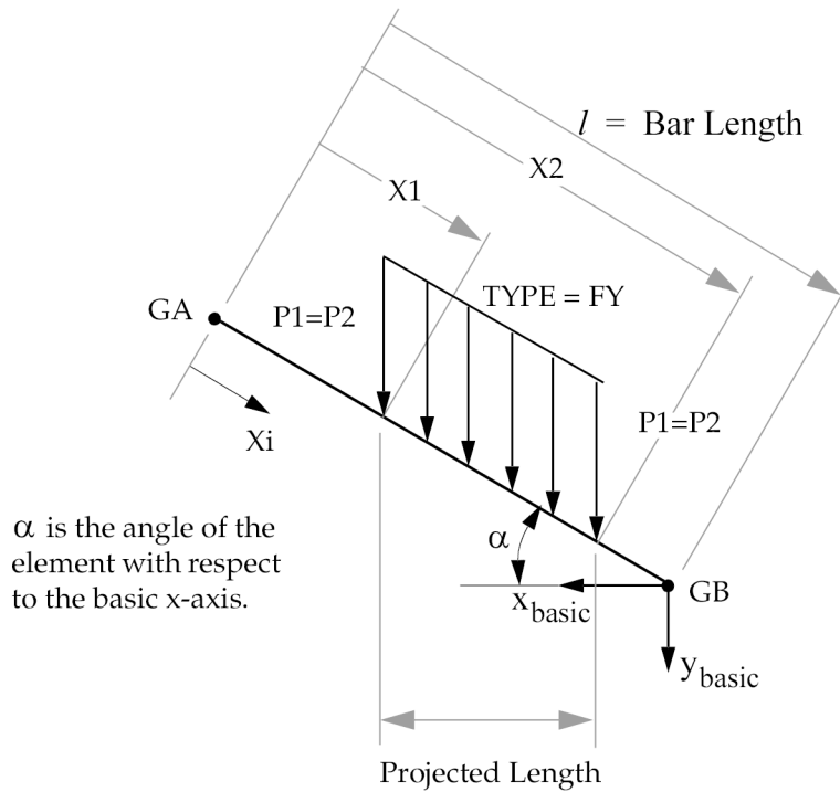
Figure 17-17. PLOAD1 Convention on Beam or Bar Elements
