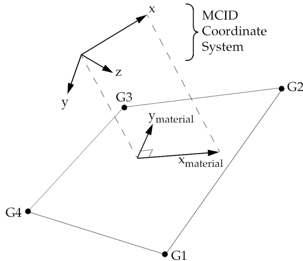
Figure 13-15. MCID Coordinate System Definition
