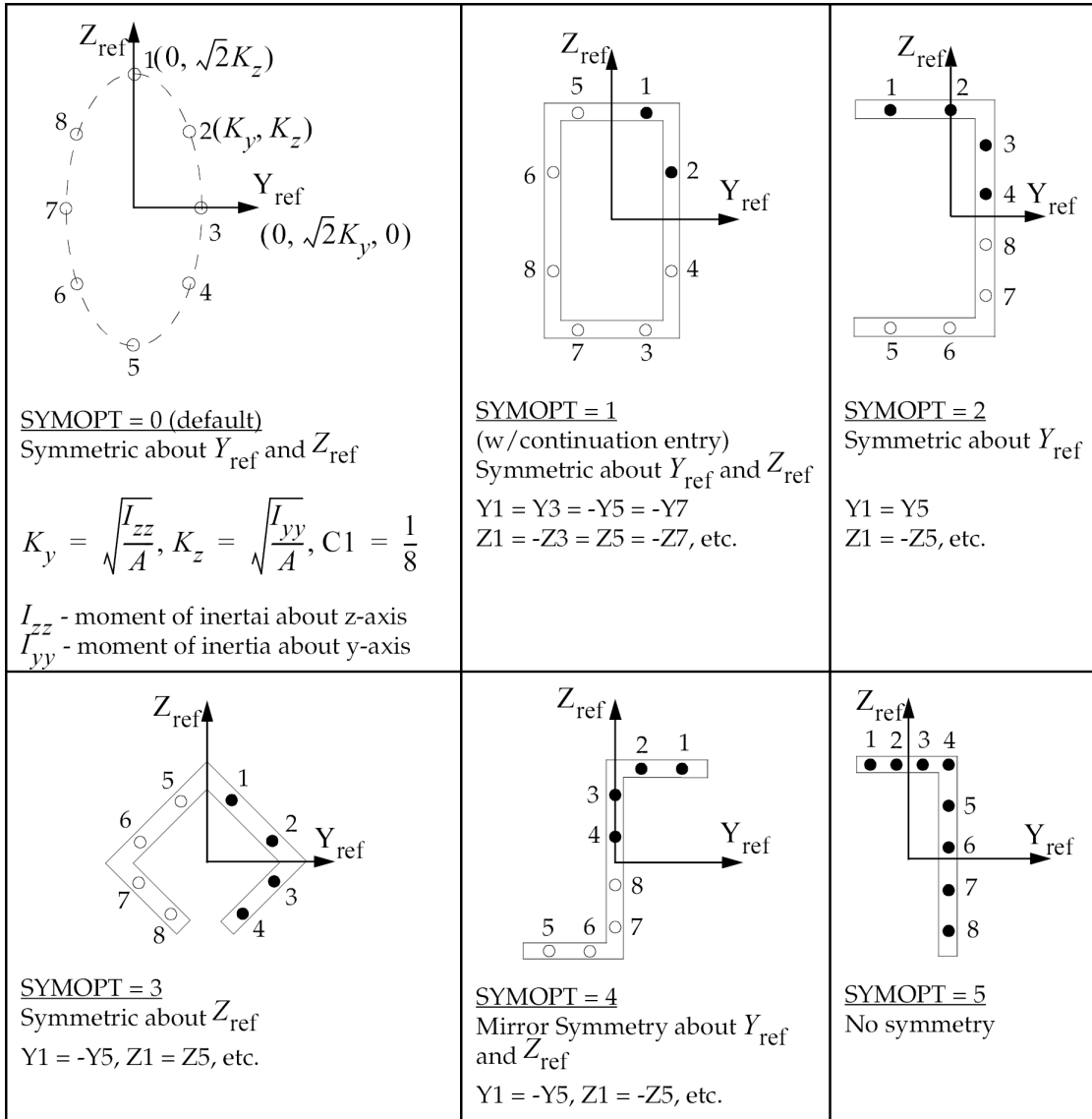
Figure 17-4. PBCOMP Entry SYMPT Type Examples with 8 Lumped Areas
