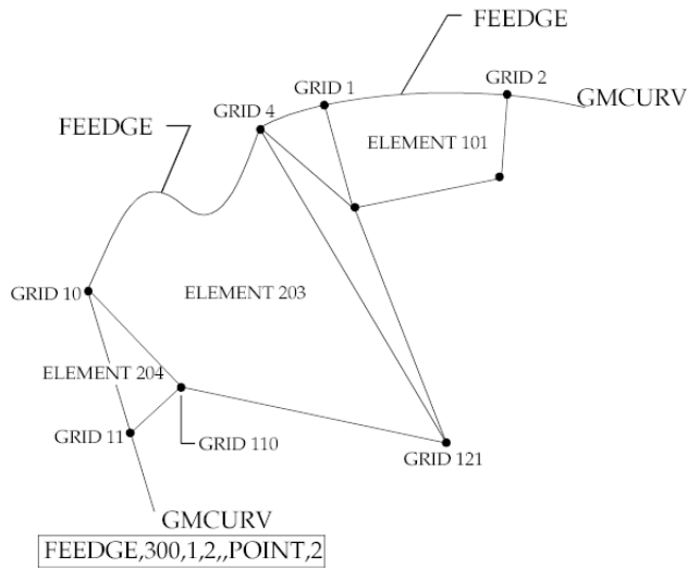
Figure 15-1. Specifying Geometry Using GEOMIN=GMCURV Method
