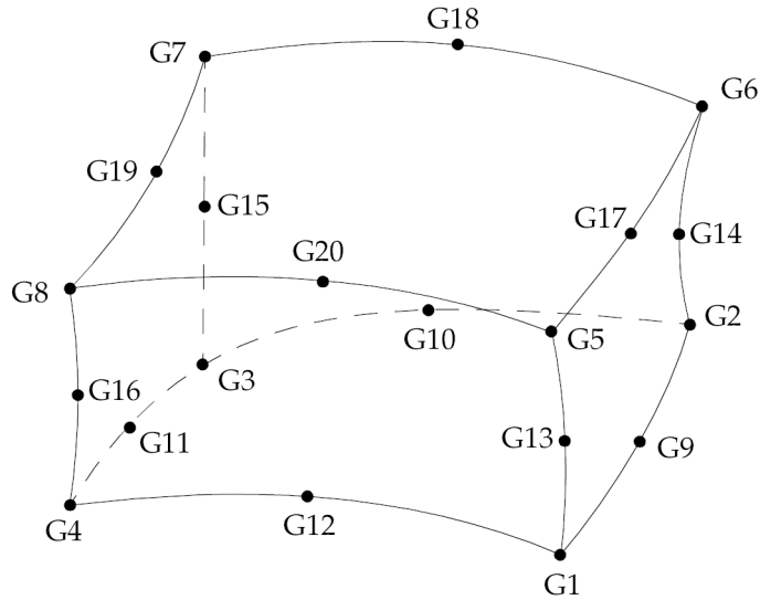
Figure 12-29. CHEXA Element Connection
