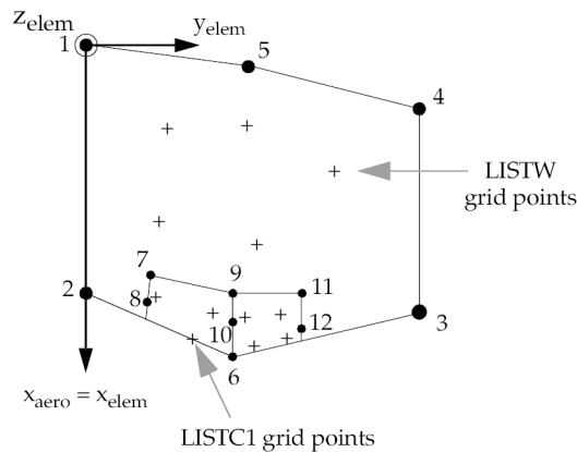
Figure 12-3. CAERO3 Element Configuration
