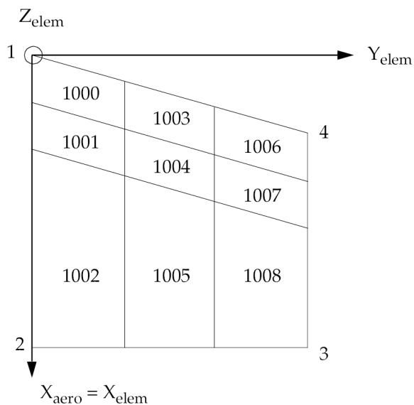
Figure 12-2. Element Coordinate System for Aerodynamic Panel
