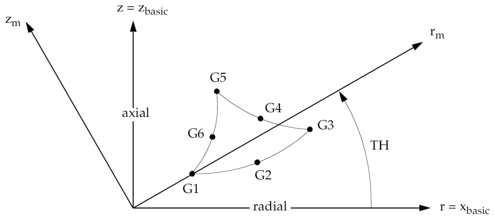
Figure 13-46. CTRIAX6 Element Geometry and Coordinate Systems
