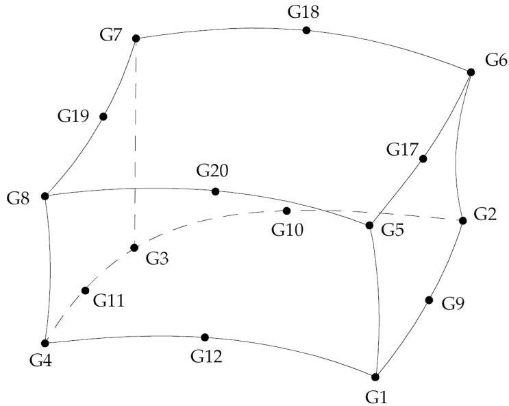
Figure 12-21. CHACAB Element Connection
