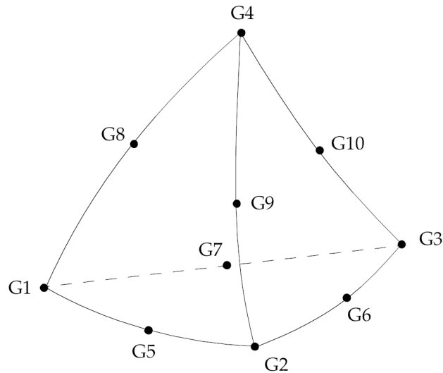
Figure 13-32. CTETRA Element Connection
