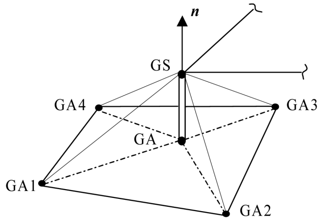
Figure 13-52. Point-to-Patch Connection Defined with Format GRIDID or ELEMID
