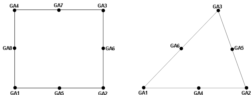
Figure 13-50. Quadrilateral and Triangular Surface Patches Defined with Format GRIDID
