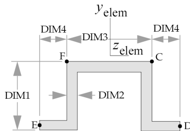
TYPE="HAT"
