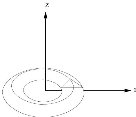
Figure 13-45. CTRIAX6 Element Idealization
