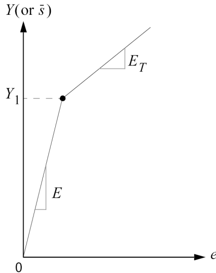
Figure 16-3. Stress-Strain Curve Definition When H Is Specified in Field 5
