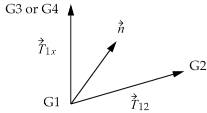
Figure 12-25. Normal Vector for CHBDYG Element of Types “AREAi”
