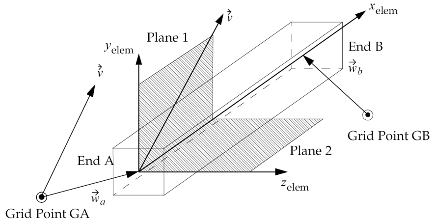
Figure 12-7. CBAR Element Geometry with Offsets
