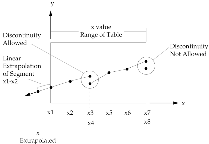
Figure 19-3. Example of Table Extrapolation and Discontinuity
