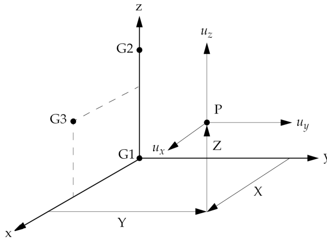
Figure 13-3. CORD1R Definition
