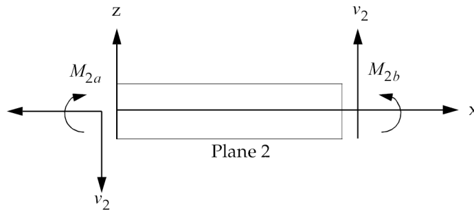
Figure 12-10. CBAR Element Internal Forces and Moments (x-z Plane)
