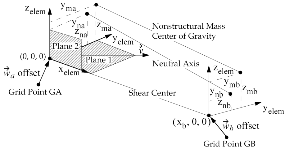
Figure 17-6. PBEAM Element Coordinate System
