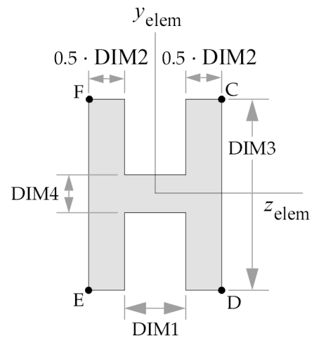
TYPE="H"
