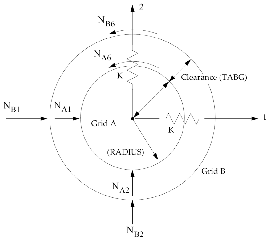
Figure 16-5. Radial Gap Orientation and Nonlinear Load Sign Conventions
