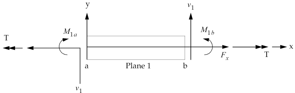
Figure 12-9. CBAR Element Internal Forces and Moments (x-y Plane)
