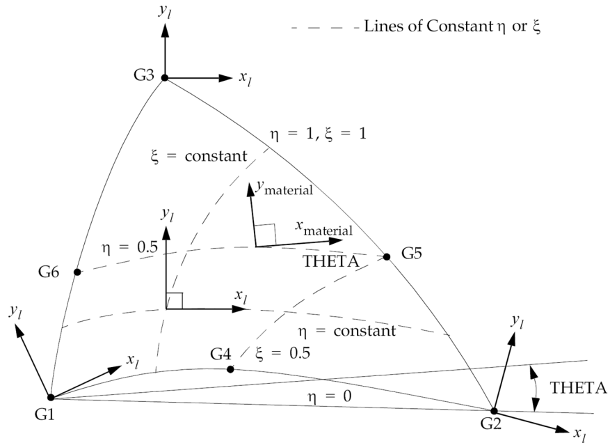
Figure 13-41. CTRIA6 Element Geometry and Coordinate Systems
