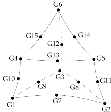
Figure 13-8. CPENTA Element Connection
