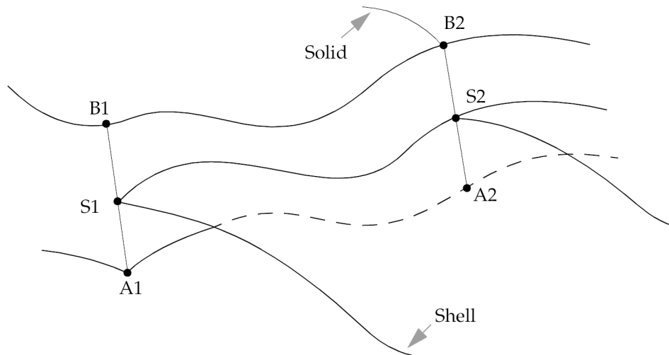
Figure 18-3. Shell Elements Connected to the Faces of Solid Elements
