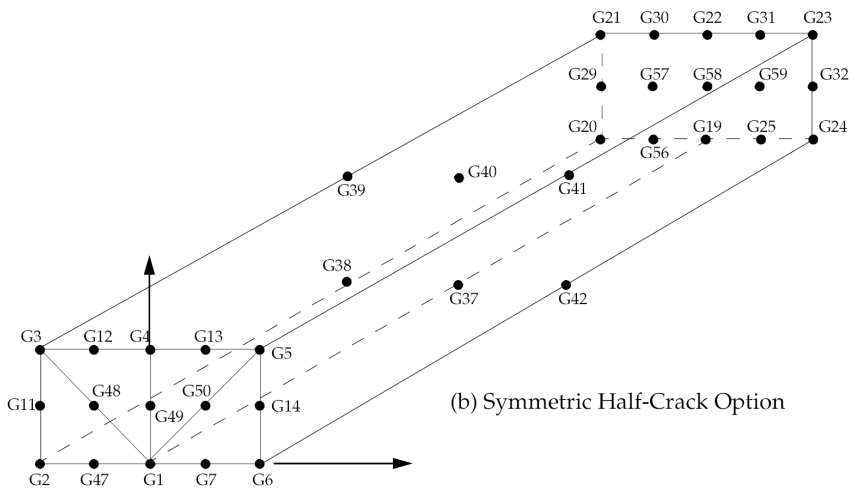
Figure 13-24. CRAC2D Solid Crack Tip Element with All Connection Points
