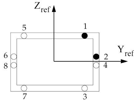
Figure 17-5. Doubly Symmetric PBCOMP Section
