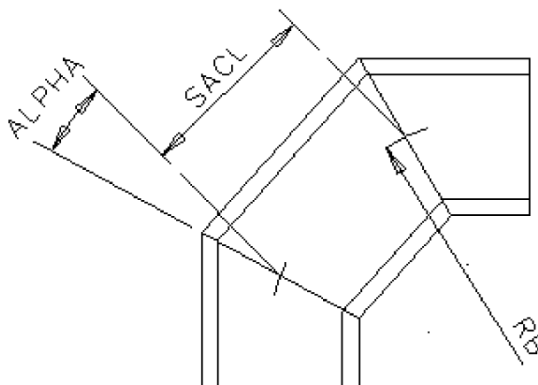
Figure 17-11. Definition of SACL and ALPHA
