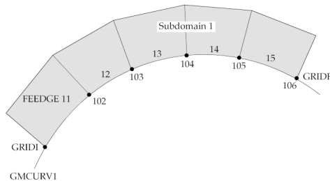
Figure 15-7. Geometric Boundary Definition
