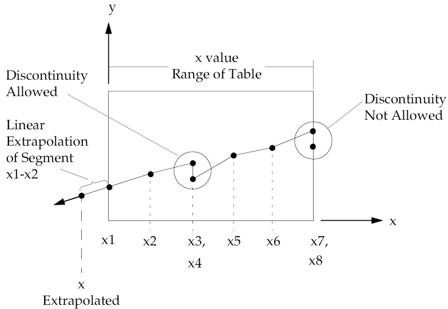
Figure 19-2. Example of Table Extrapolation and Discontinuity
