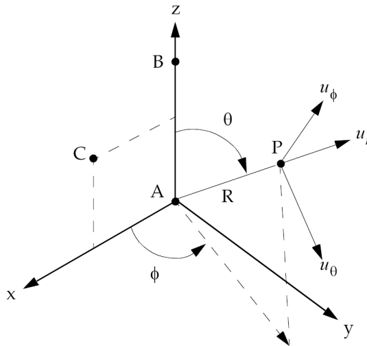
Figure 13-7. CORD2S Definition
