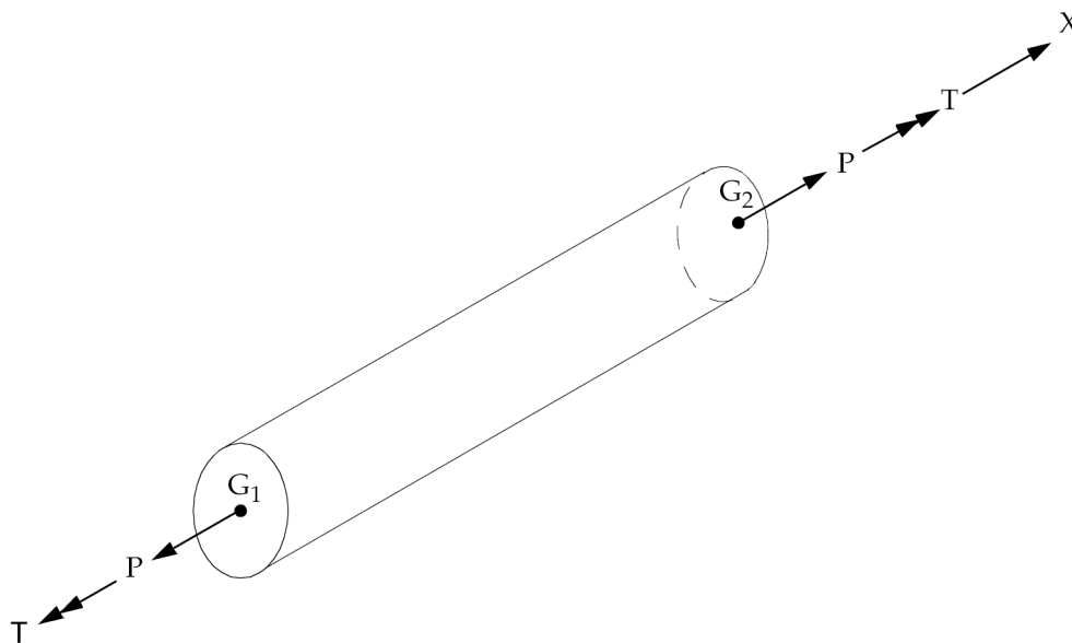
Figure 13-1. CONROD Element Forces and Moments
