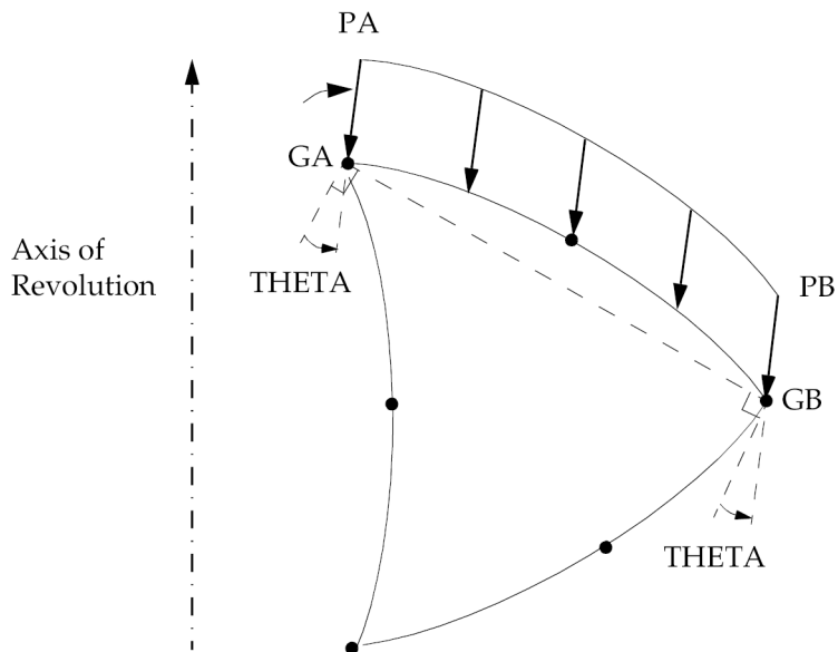
Figure 17-18. Pressure Load on CTRIA6 or CTRIA3 Element
