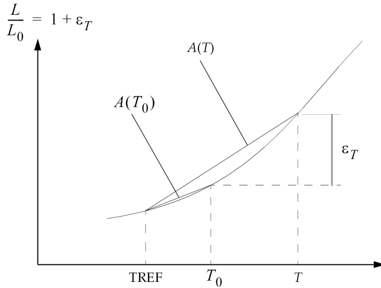
Figure 16-1. Use of TREF in Calculation of Thermal Loads
