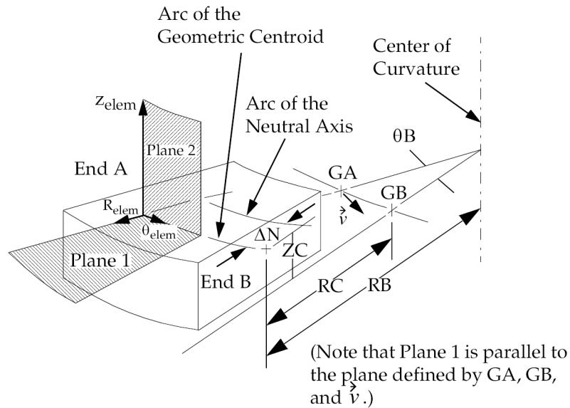
Figure 12-14. CBEND Element Coordinate System
