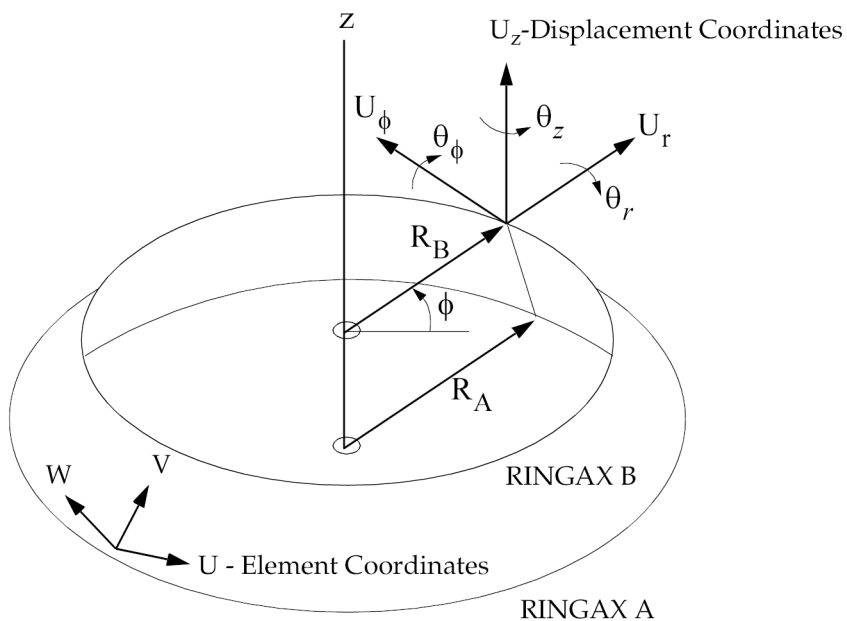
Figure 18-2. RINGAX Coordinate System
