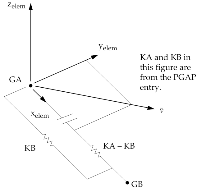
Figure 12-20. CGAP Element Coordinate System
