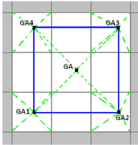
Figure 13-49. Weld Connections with Format ELPAT or PARTPAT
