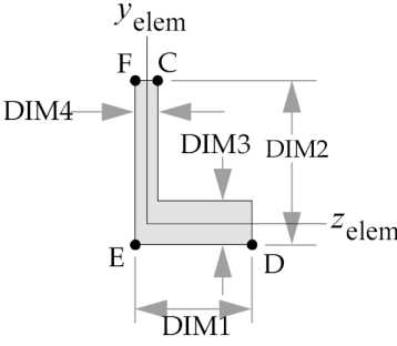
TYPE="L"
