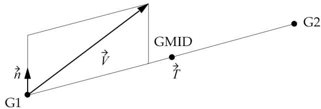
Figure 12-27. Normal Vector for CHBDYP Element with TYPE=“LINE”,TYPE=“FTUBE”, or TYPE=“TUBE”(See Remarks 4 and 5.)
