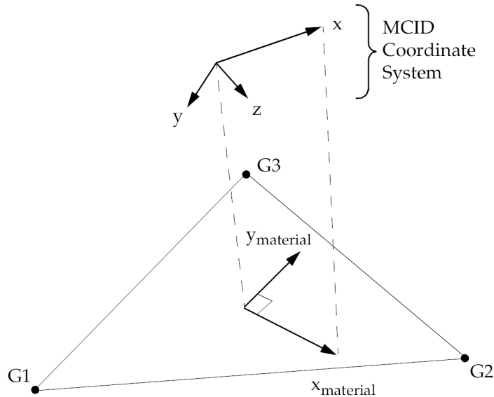
Figure 13-42. MCID Coordinate System Definition
