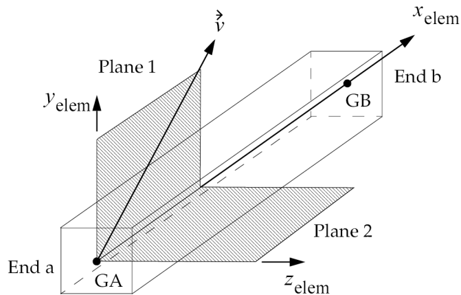
Figure 17-2. PBAR Element Coordinate System
