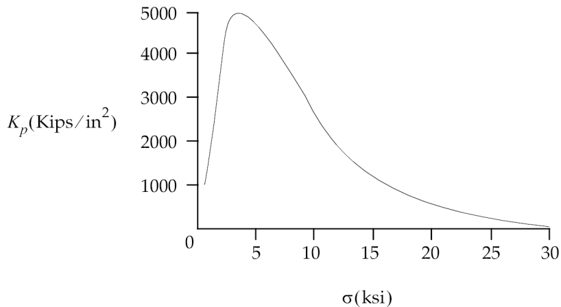
Figure 13-26. $K_p$ Versus $\sigma$ Example for CREEP
