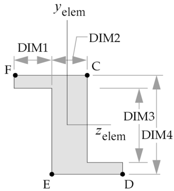
TYPE="Z"
