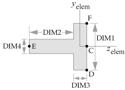
TYPE="T1"
