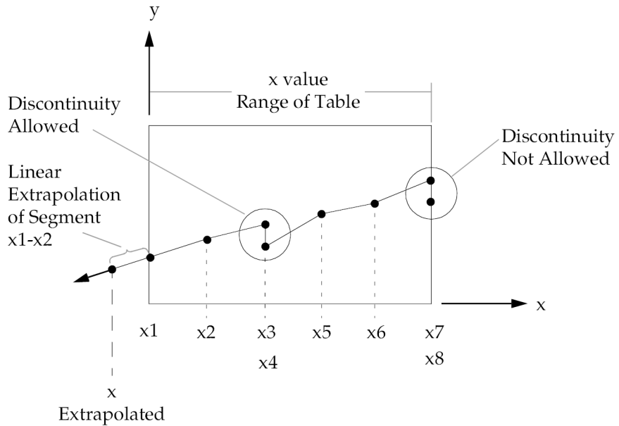
Figure 19-6. Example of Table Extrapolation and Discontinuity
