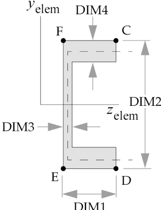
TYPE="CHAN"
