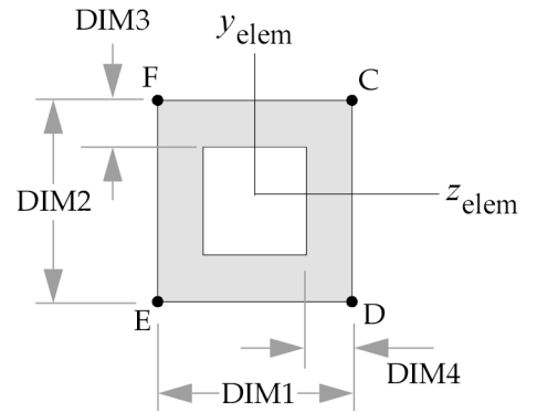
TYPE="BOX"
