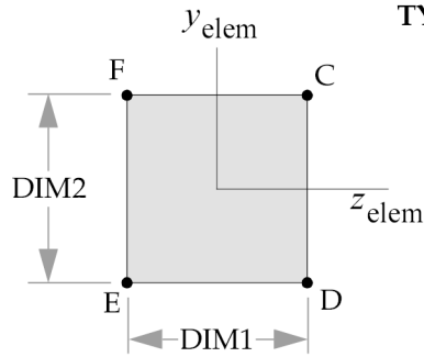
TYPE="BAR"
