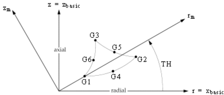
Figure 13-37. CTRAX6 Element Geometry and Coordinate Systems
