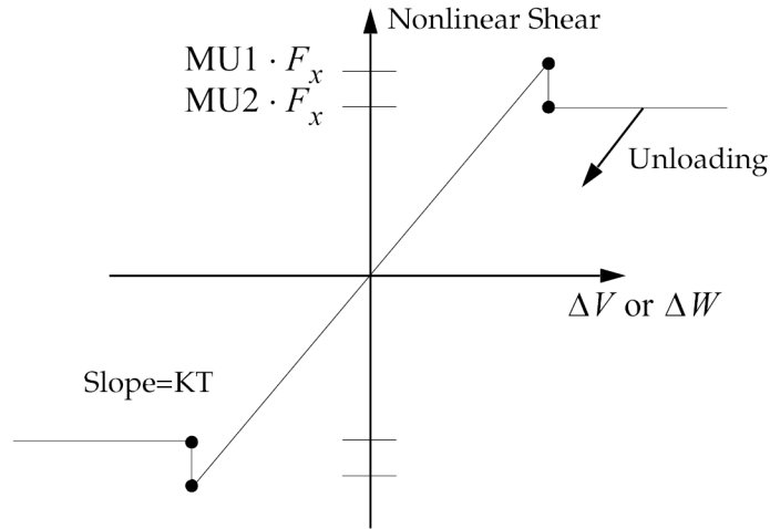
Figure 17-14. Shear Force for CGAP Element
