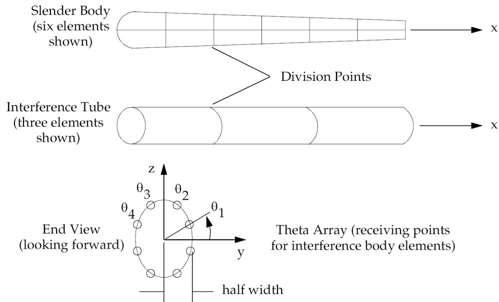
Figure 17-1. Idealization of Aerodynamic Body
