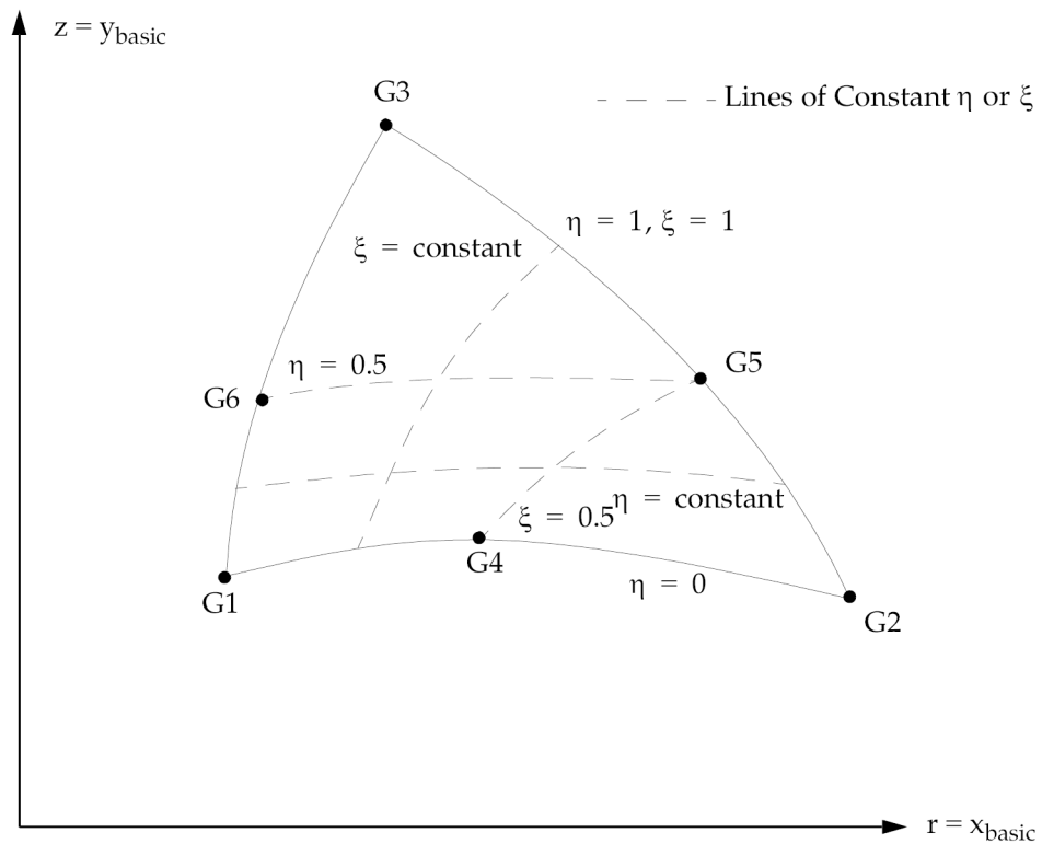
Figure 13-44. CTRIAX Element Coordinate System
