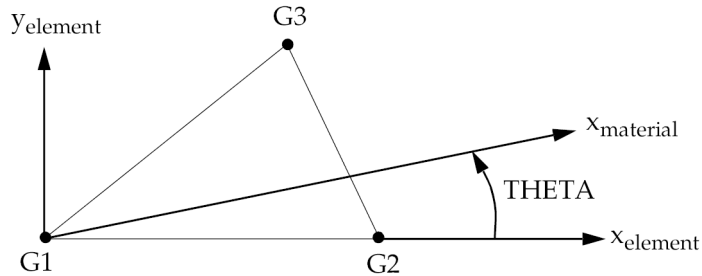
Figure 13-39. CTRIA3 Element Geometry and Coordinate Systems
