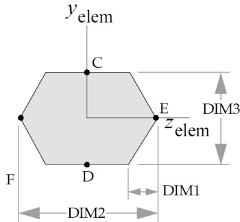
TYPE="HEXA"
