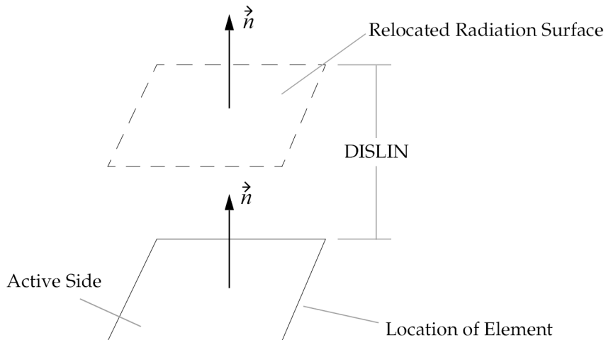
Figure 19-10. DISLIN Convention
