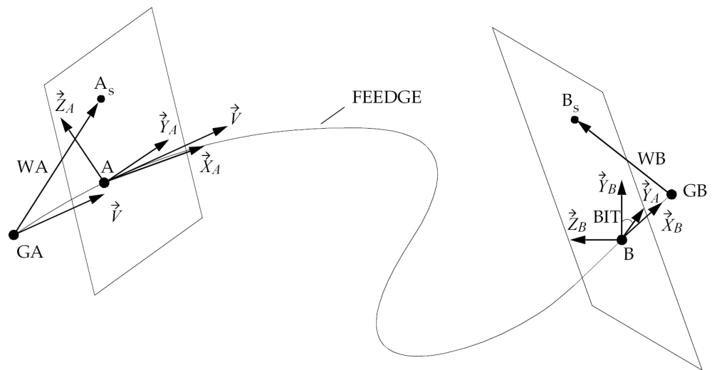
Figure 12-12. CBEAM Element Geometry System (p-adaptive)
