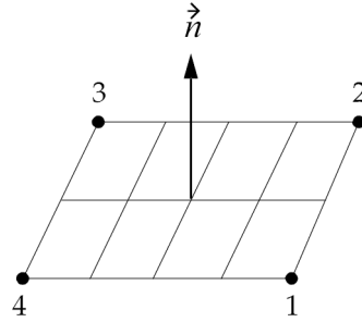
Figure 19-11. Typical AREA4 surface element where NB=2 and NG=4
