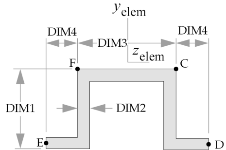
TYPE="HAT"
