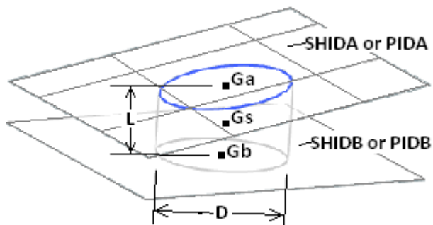
Figure 13-47. Patch-to-Patch Connection Defined with Format ELPAT or PARTPAT
