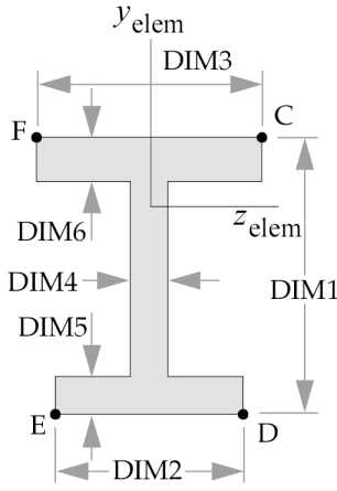
TYPE="I"
