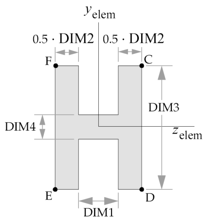
TYPE="H"
