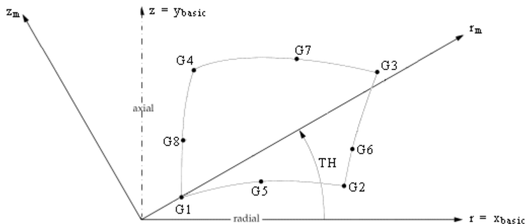
Figure 13-21. CQUADX8 Element Geometry and Coordinate Systems
