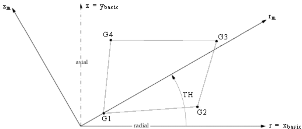
Figure 13-19. CQUADX4 Element Geometry and Coordinate Systems
