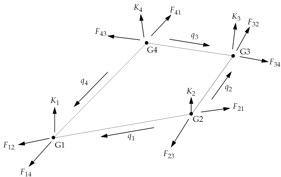
Figure 13-31. CSHEAR Element Corner Forces and Shear Flows
