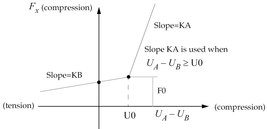
Figure 17-13. CGAP Element Force-Deflection Curve for Nonlinear Analysis
