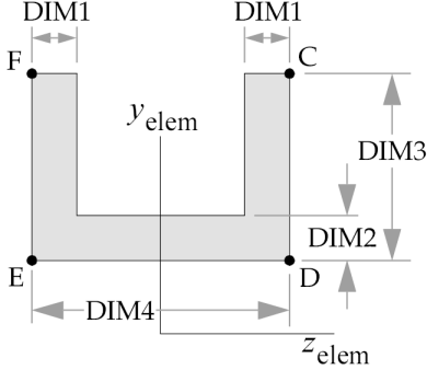
TYPE="CHAN2"
