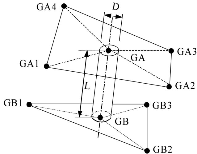
Figure 17-21. Length and Diameter of the Weld Connector
