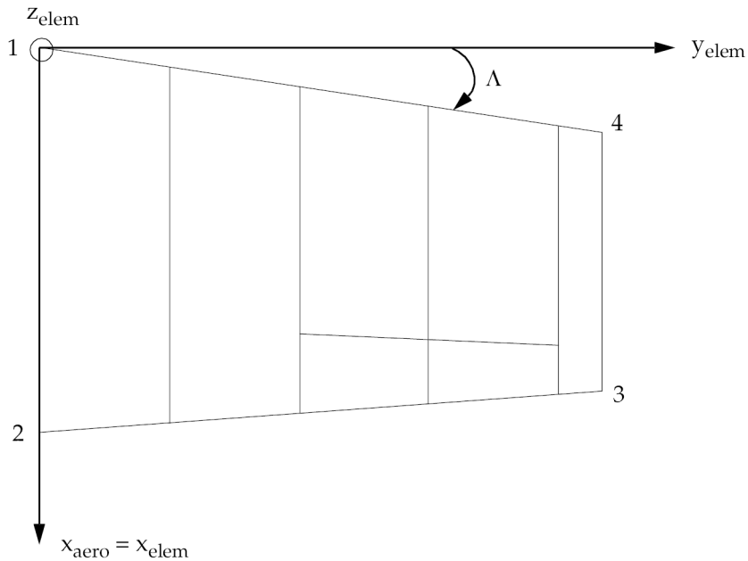
Figure 12-5. CAERO5 Element Configuration
