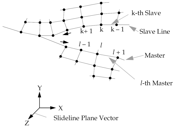
Figure 11-1. A Typical Finite Element Slideline Contact Region
