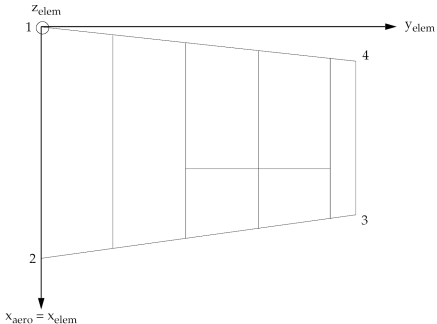
Figure 12-4. CAERO4 Element Connection
