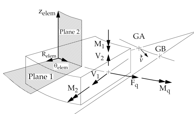
Figure 12-15. CBEND Element Internal Forces and Moments
