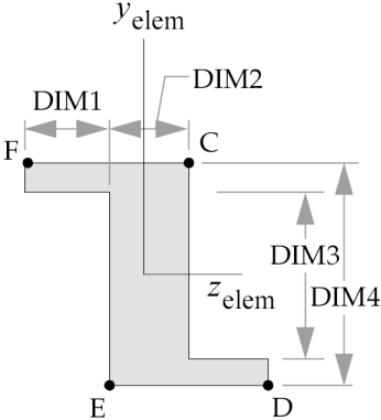
TYPE="Z"
