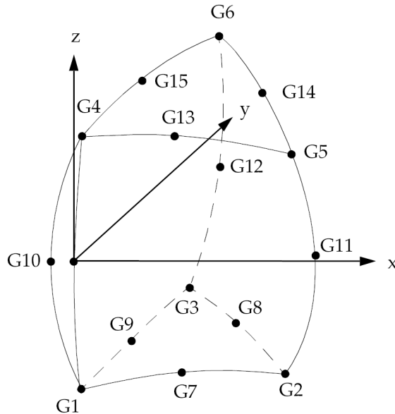
Figure 13-9. CPENTA Element Coordinate System
