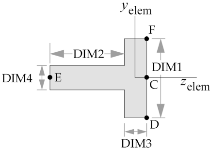
TYPE="T1"
