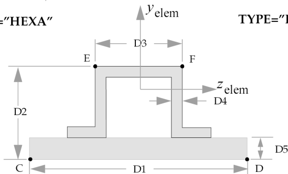
TYPE="HAT1"
