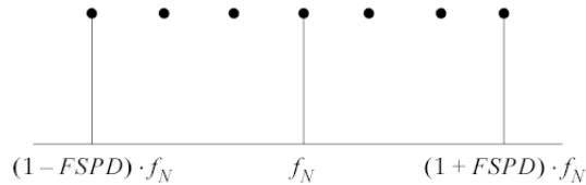
Figure 15-4. Frequency Spread Definition
