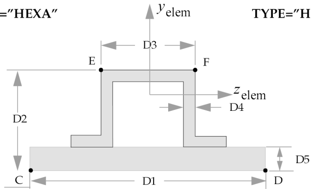
TYPE="HAT1"
