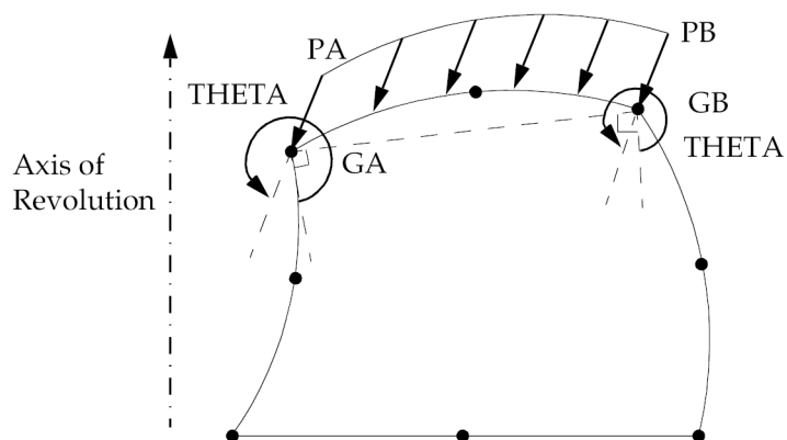
Figure 17-19. Pressure Load on CQUADX Element
