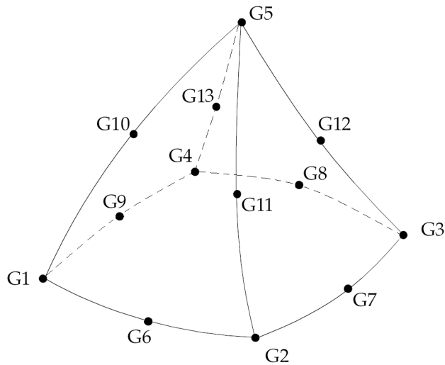
Figure 13-10. CPYRAM Element Connection
