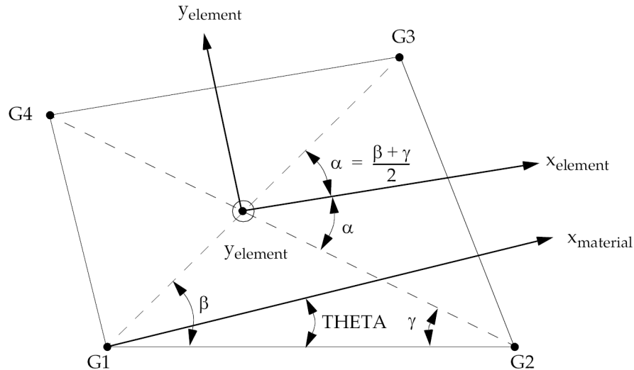
Figure 13-13. CQUAD4 Element Geometry and Coordinate Systems
