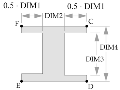
TYPE="I1"
