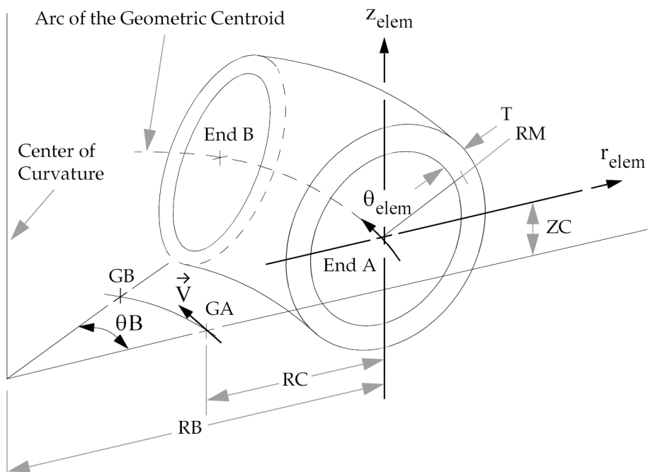
Figure 17-10. PBEND Circular Cross Section Element Coordinate System
