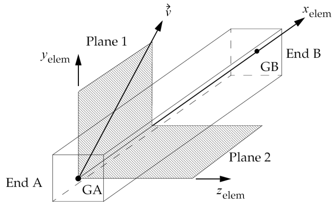
Figure 12-8. CBAR Element Geometry without Offsets
