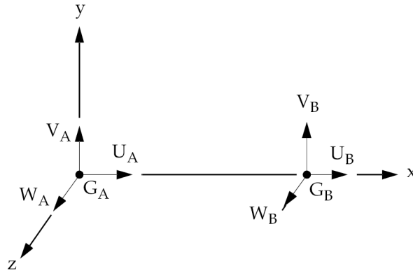
Figure 17-12. The CGAP Element Coordinate System
