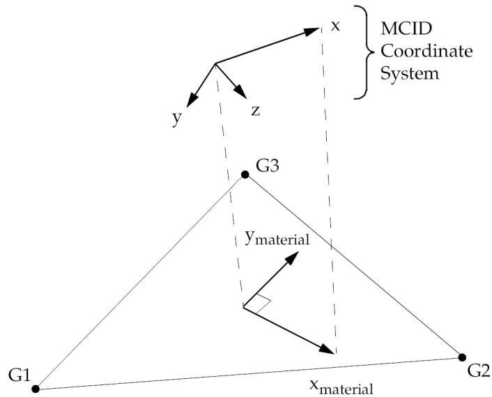
Figure 13-38. MCID Coordinate System Definition
