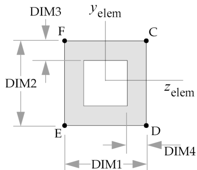
TYPE="BOX"
