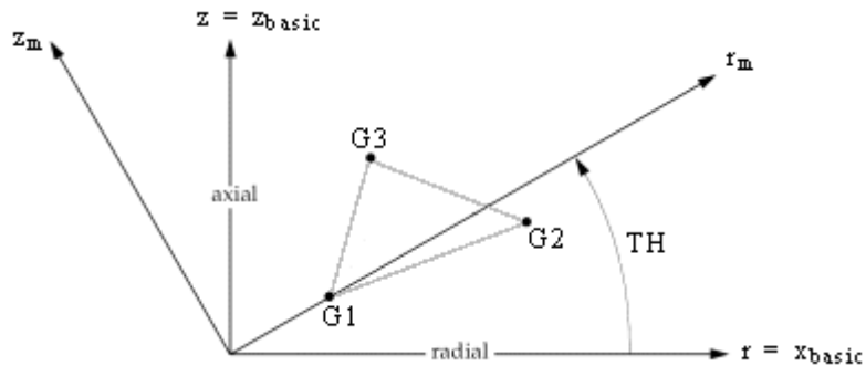
Figure 13-35. CTRAX3 Element Geometry and Coordinate Systems
