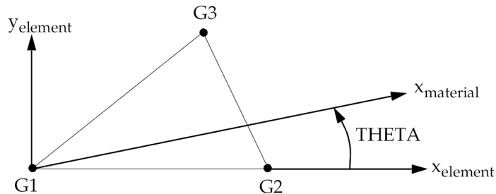
Figure 13-43. CTRIAR Element Geometry and Coordinate Systems
