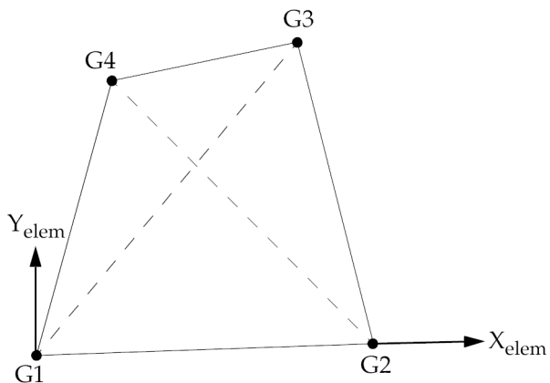
Figure 13-30. CSHEAR Element Connection and Coordinate System
