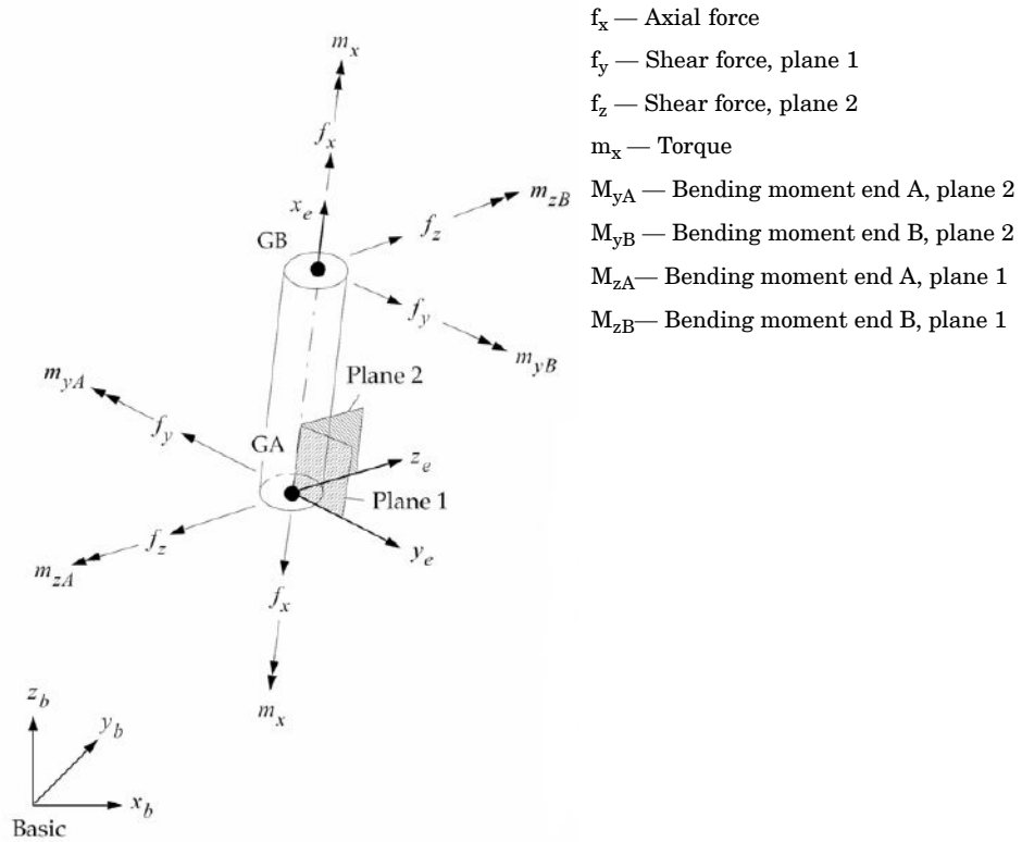
Figure 13-54. Element Coordinate System and Sign Convention of Element Forces
