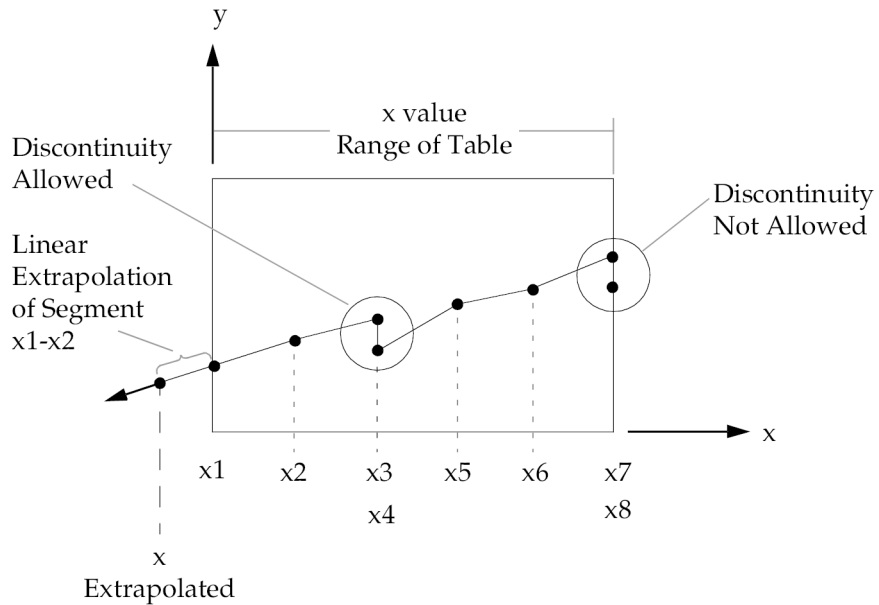
Figure 19-7. Example of Table Extrapolation and Discontinuity
