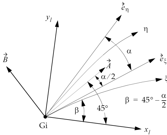
Figure 13-14. CQUAD8 Element Geometry and Coordinate Systems
