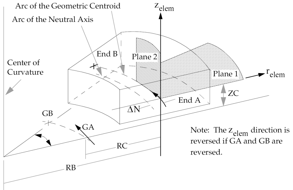
Figure 17-9. PBEND Element Coordinate System
