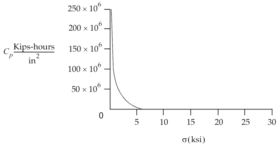
Figure 13-27. C p Versus s Example for CREEP
