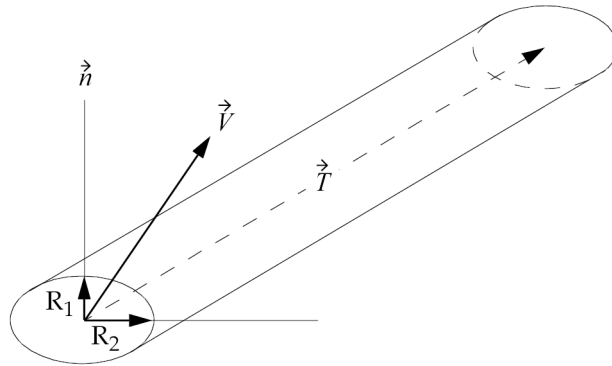
Figure 12-28. Normal Vector for CHBDYP Element of TYPE="ELCYL"(See Remarks 4 and 5.)
