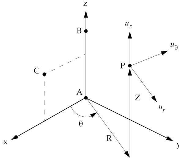
Figure 13-5. CORD2C Definition
