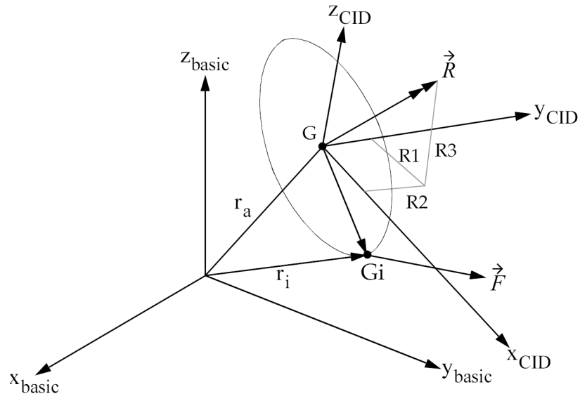
Figure 18-1. RFORCE Vector at Grid Point Gi
